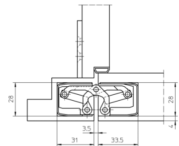
Futterzarge
