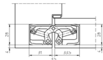
Blockzarge
