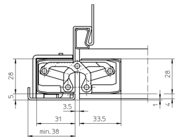
Stahlzarge
